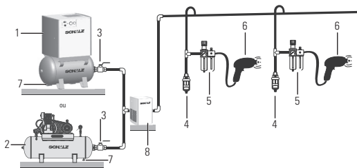
FIGURE 1 - INSTALLATION SETUP GUIDE
