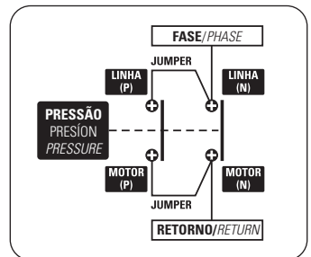
MONOFÁSICO INGLE-PHASE
