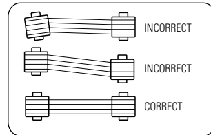
FIGURE 7.16 - PULLEY ALIGNMENT
